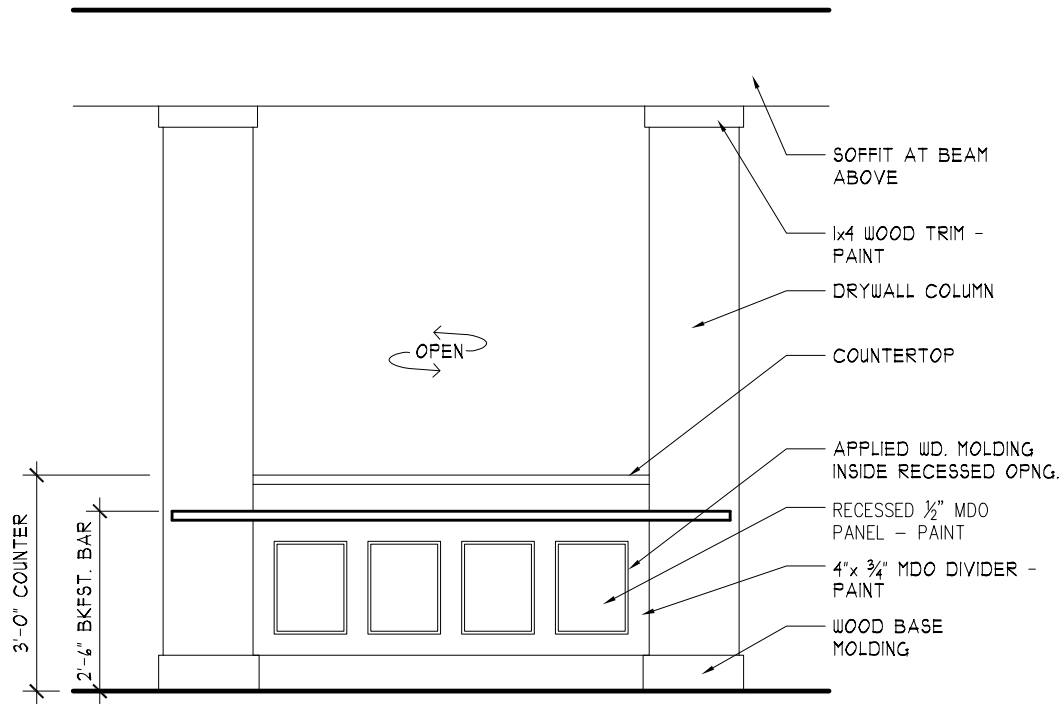
BACK SIDE OF ISLAND (DETAIL 1 of 3)
